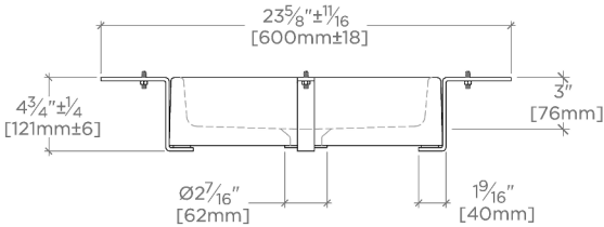
FRONT VIEW SCALE: 1"=1'-0"
