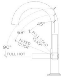
HANDLE OPERATION
