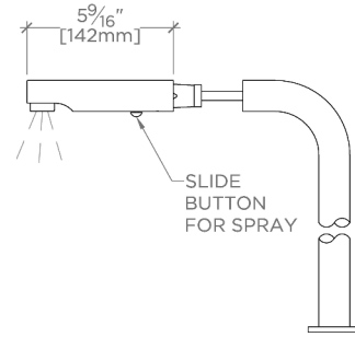
SPRAY OPERATION
