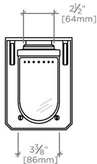
FRONT VIEW SCALE: 1/2"=1'-0"
