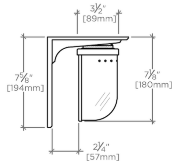
SIDE VIEW SCALE: 1/2"=1'-0"
