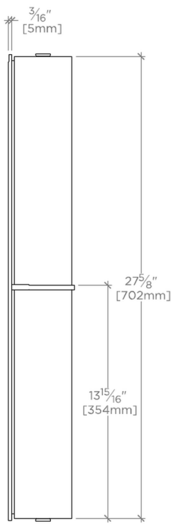
SIDE VIEW SCALE: 1 1/2"=1'-0"
