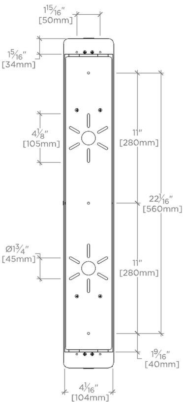
MOUNTING PLATE SCALE: 1 1/2"=1'-0"
