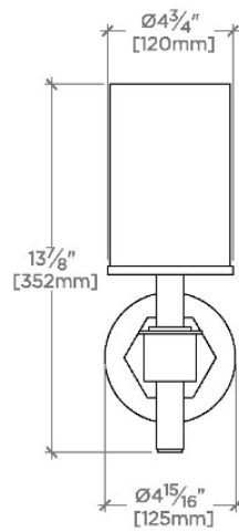
FRONT VIEW SCALE: 1 1/2"=1'-0"
