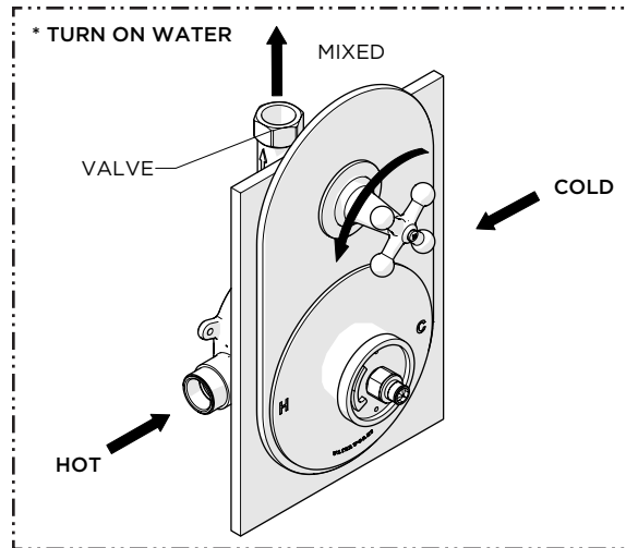
17. Turn on the water supply and open the VOLUME CONTROL VALVE to run water through the THERMOSTATIC VALVE.
