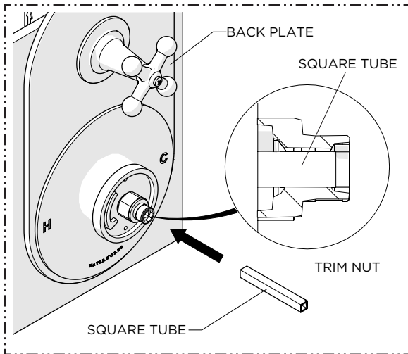
16. Mark the SQUARE TUBE where it passes through the front face of the TRIM NUT then remove and cut the TUBE 1/8" [3mm] behind the previous mark.
