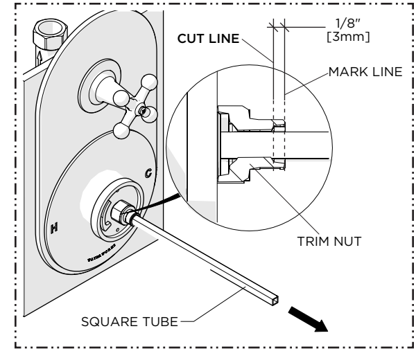
15. Mark the SQUARE TUBE where it passes through the front face of the TRIM NUT then remove and cut the TUBE 1/8" [3mm] behind the previous mark.
