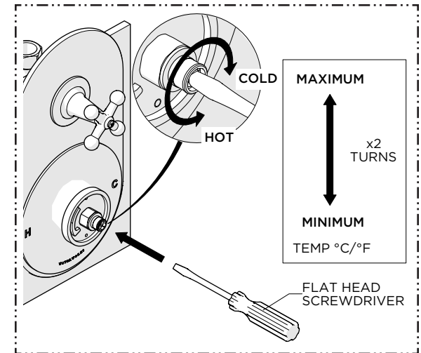
18. Insert a bladed screw driver into the SQUARE TUBE. Slowly rotate the TUBE clockwise to attain full cold then counterclockwise to attain full hot. It's approximately 2 complete rotations. Verify a full range of temperatures exists.
