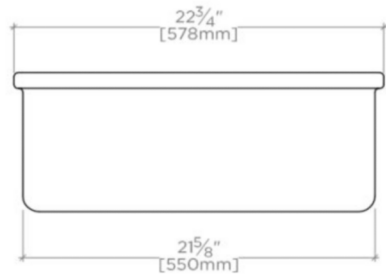
FRONT VIEW SCALE: 1"=1'-0"
