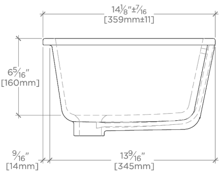
SIDE VIEW SCALE: 1 1/2"=1'-0"
