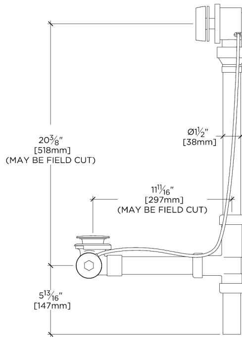
SIDE VIEW SCALE: 1 1/2"=1'-0"
