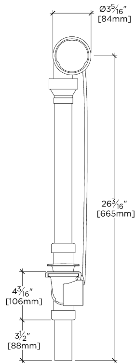
FRONT VIEW SCALE: 1 1/2"=1'-0"
