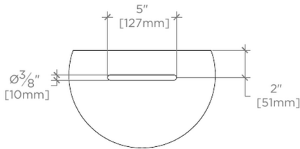
OVERFLOW DETAIL
