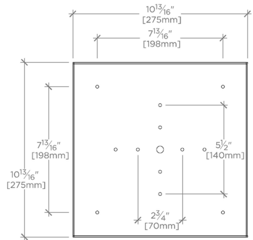
MOUNTING PLATE
