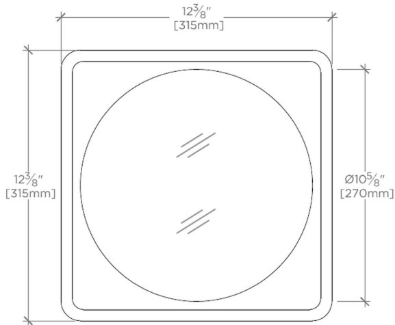
CEILING VIEW
