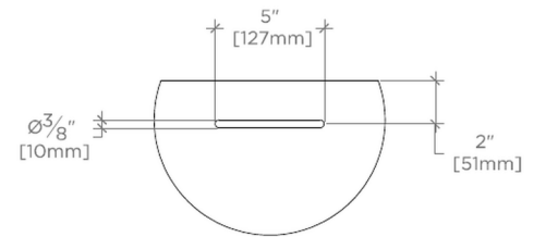
OVERFLOW DETAILS
