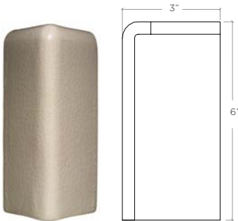
MUD CAP OUTCORNER 3" X 6" ARMU03
