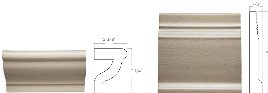
METROPOLIS CROWN 3 1/4" X 6" ARCW5E
