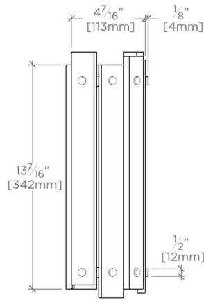
SIDE VIEW SCALE: 1 1/2"=1'-0"
