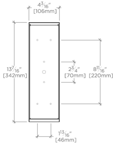
MOUNTING PLATE SCALE: 1 1/2"=1'-0"
