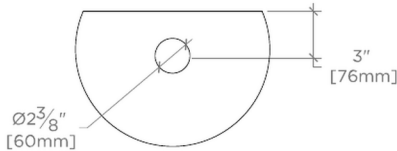
OVERFLOW DETAIL
