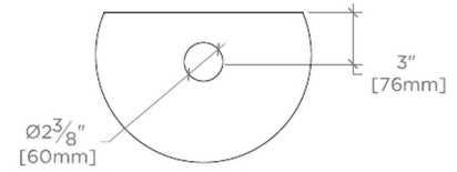
OVERFLOW DETAIL
