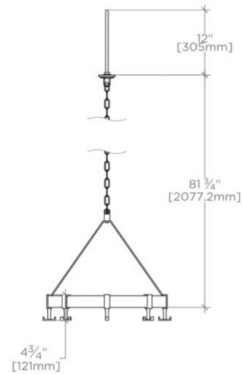
END VIEW
