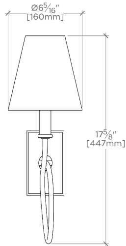
FRONT VIEW SCALE: 1\frac{1}{2}"=1'-0"
