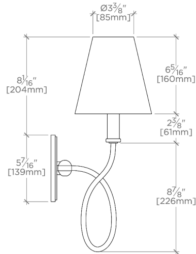
SIDE VIEW SCALE: 1\frac{1}{2}"=1'-0"
