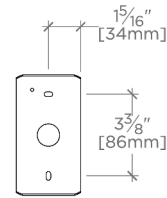
MOUNTING PLATE SCALE: 1\frac{1}{2}"=1'-0"
