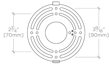
MOUNTING PLATE
