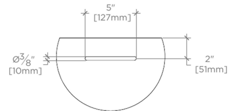
OVERFLOW DETAIL
