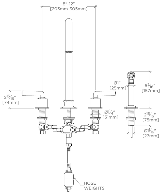
FRONT VIEW
