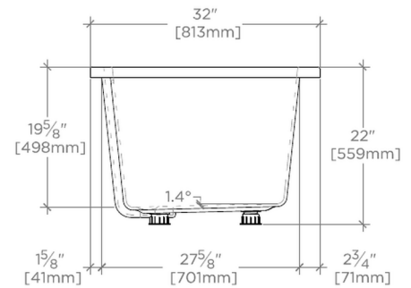
END VIEW
