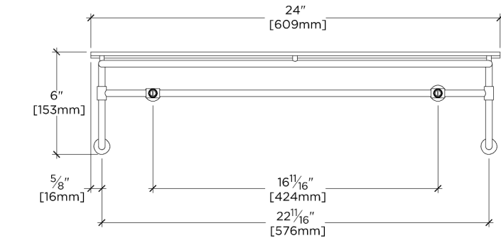
FRONT VIEW SCALE: 1 1/2"=1'-0"
