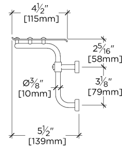
SIDE VIEW SCALE: 1 1/2"=1'-0"
