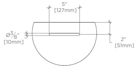
OVERFLOW DETAIL
