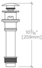
FRONT VIEW SCALE: 1 1/2"=1'-0"
