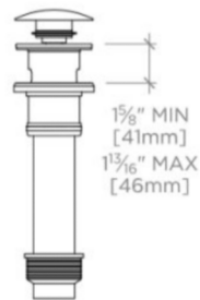
SIDE VIEW SCALE: 1 1/2"=1'-0"
