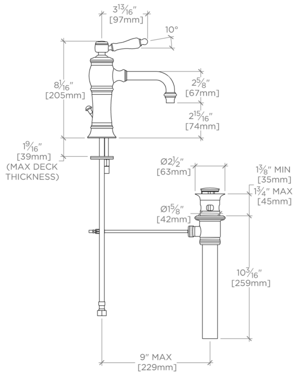
SIDE VIEW SCALE: 1 1/2"=1'-0"
