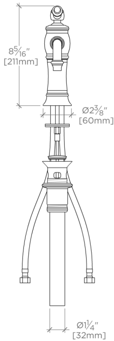
FRONT VIEW SCALE: 1 1/2"=1'-0"
