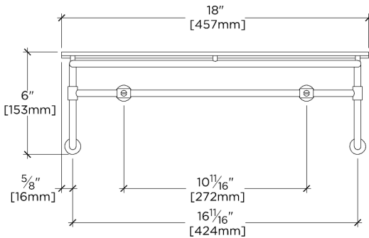
FRONT VIEW SCALE: 1 1/2"=1'-0"
