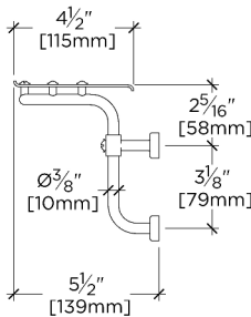
SIDE VIEW SCALE: 1 1/2"=1'-0"
