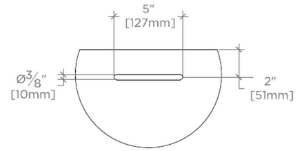
OVERFLOW DETAIL
