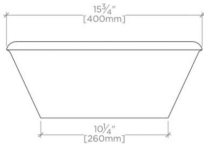
FRONT VIEW SCALE: 1 1/2"=1'-0"
