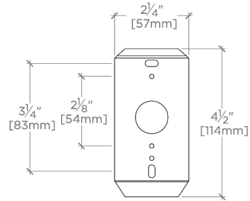
MOUNTING PLATE
