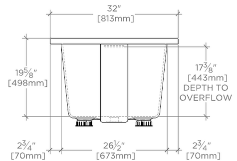
END VIEW
