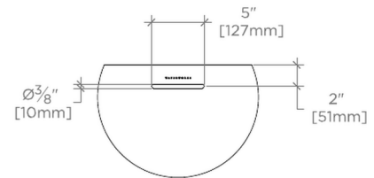
OVERFLOW DETAIL
