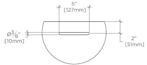
OVERFLOW DETAIL
