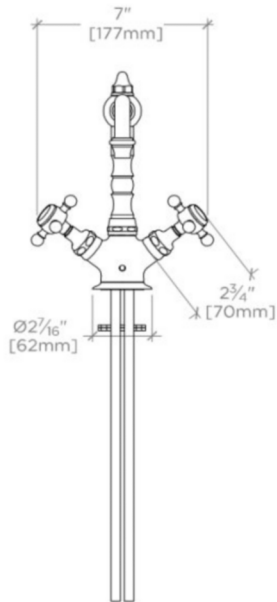
FRONT VIEW SCALE: 1 1/2"=1'-0"
