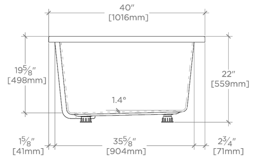
END VIEW
