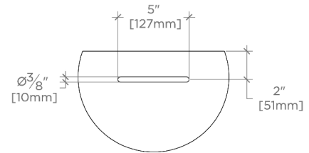
OVERFLOW DETAIL
