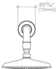
FRONT VIEW SCALE: 1 1/2"=1'-0"
