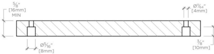
RECOMMENDED CABINET DRILLING
