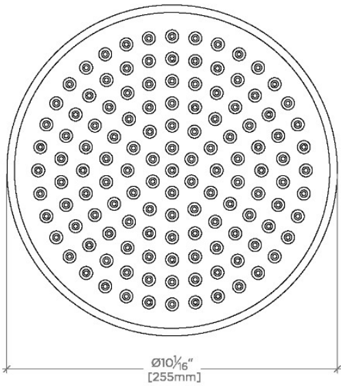
CEILING VIEW
