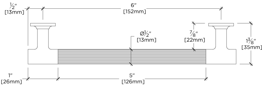
TOP VIEW
