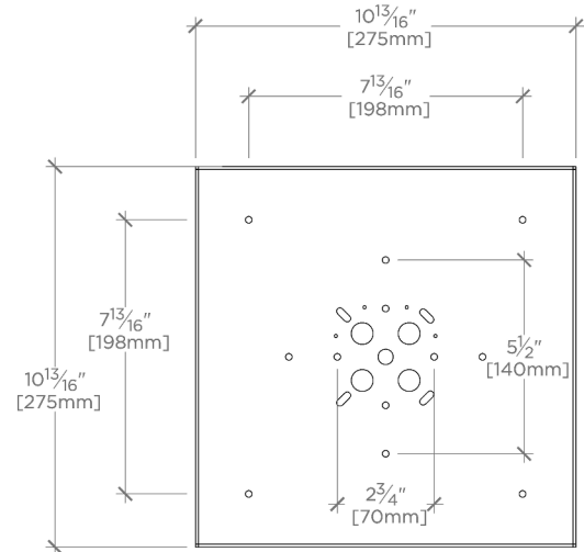
MOUNTING PLATE
