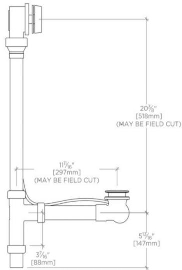
SIDE VIEW SCALE: 1 1/2"=1'-0"
