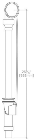
FRONT VIEW SCALE: 1 1/2"=1'-0"
