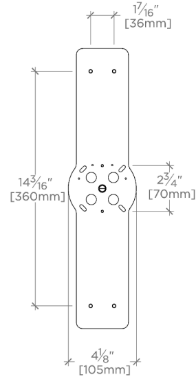
MOUNTING PLATE SCALE: 1 1/2"=1'-0"
