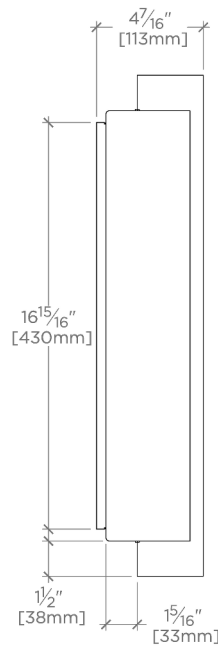
SIDE VIEW SCALE: 1 1/2"=1'-0"
