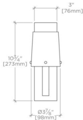
FRONT VIEW SCALE: 1/2"=1'-0"
