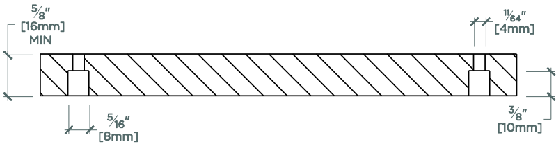
RECOMMENDED CABINET DRILLING SCALE: 6"=1'-0"
