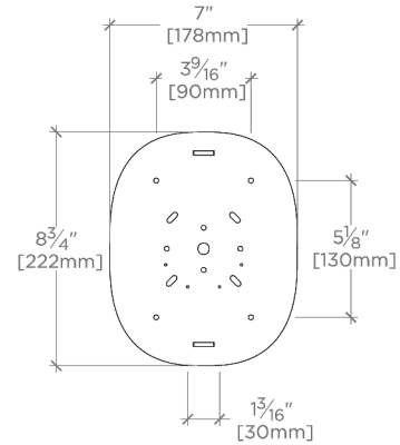
MOUNTING PLATE
