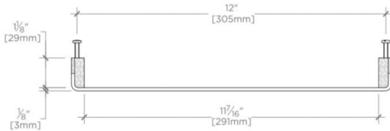
TOP VIEW
