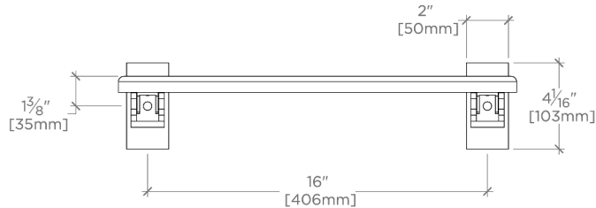
FRONT VIEW SCALE: 1 1/2" = 1'-0"
