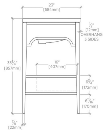
SIDE VIEW SCALE: 3/4"=1'-0"
