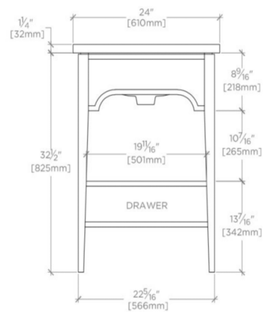
FRONT VIEW SCALE: 3/4"=1'-0"
