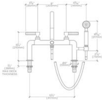
FRONT VIEW SCALE: 3/4"=1'-0"
