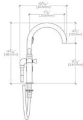
SIDE VIEW SCALE: 3/4"=1'-0"
