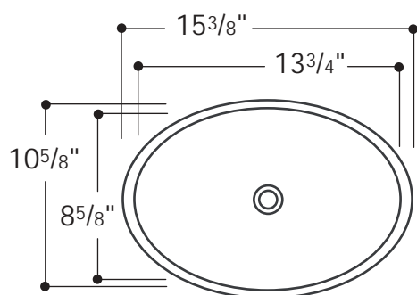
Oval Lavatory NOLV35
