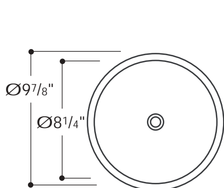
Round Lavatory NOLV45
