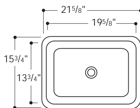
Farmhouse Lavatory NOLV23
