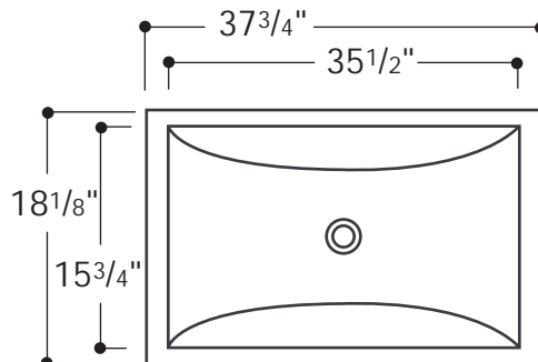
Rectangular Lavatory NOLV55
