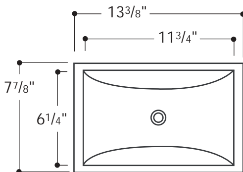
Rectangular Lavatory NOLV59
