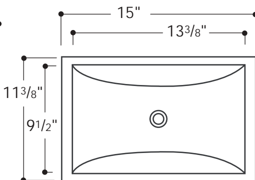
Rectangular Lavatory NOLV57
